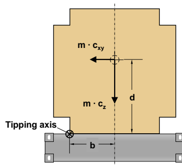
Figure 7.37 Tipping criterion
